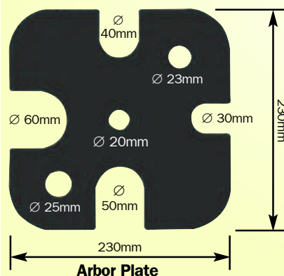
Arbor Plate
